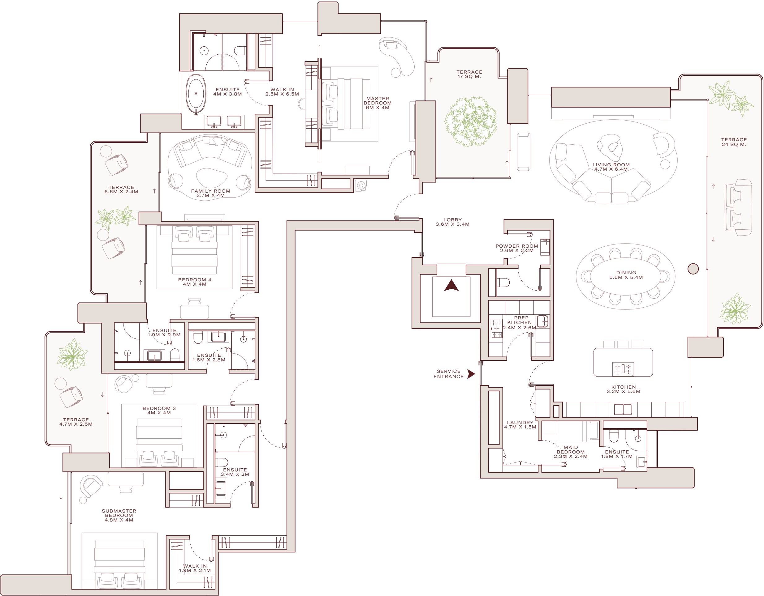
BUILDING FLOORPLATE
