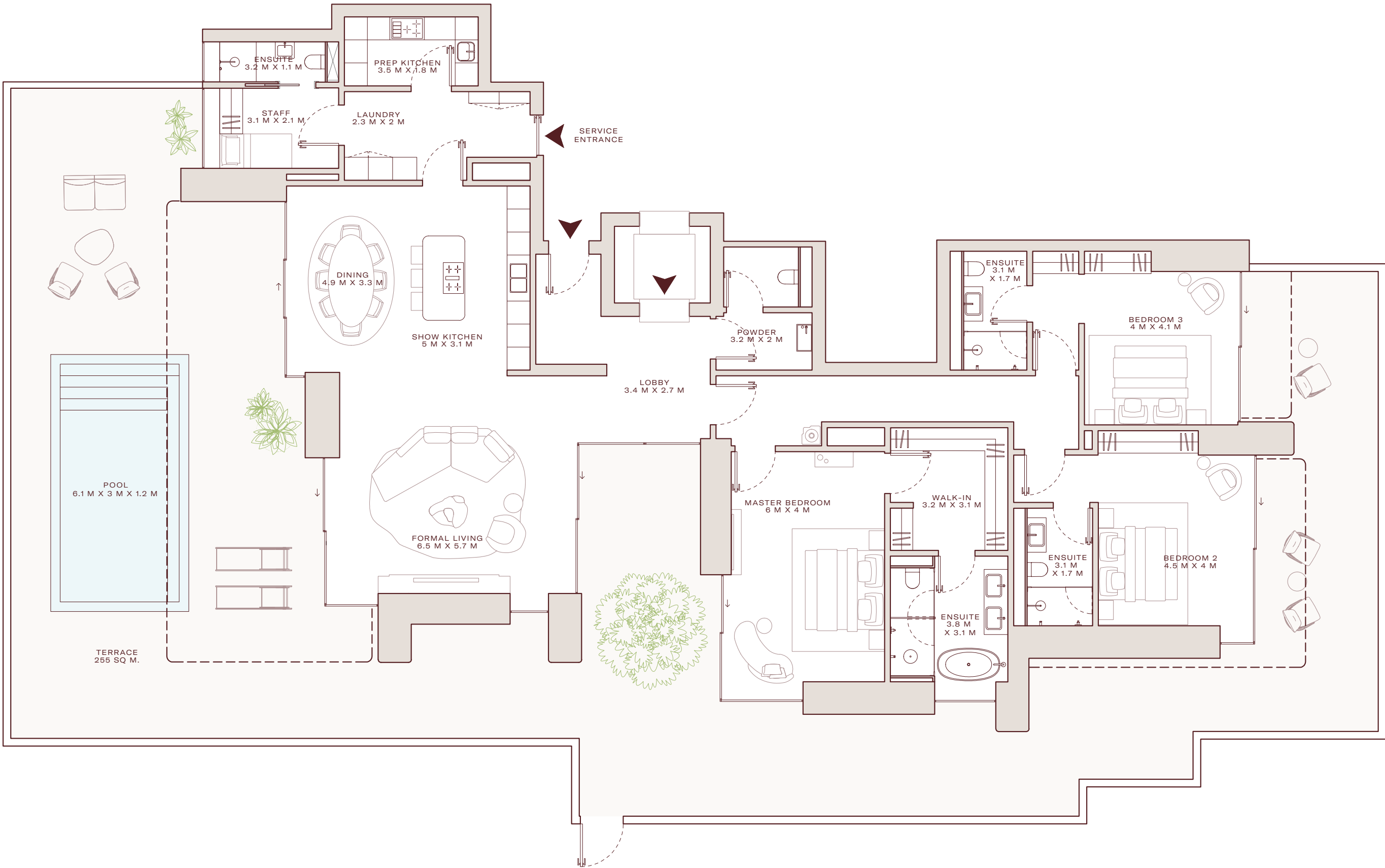
BUILDING FLOORPLATE
